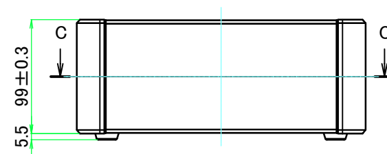
A view
